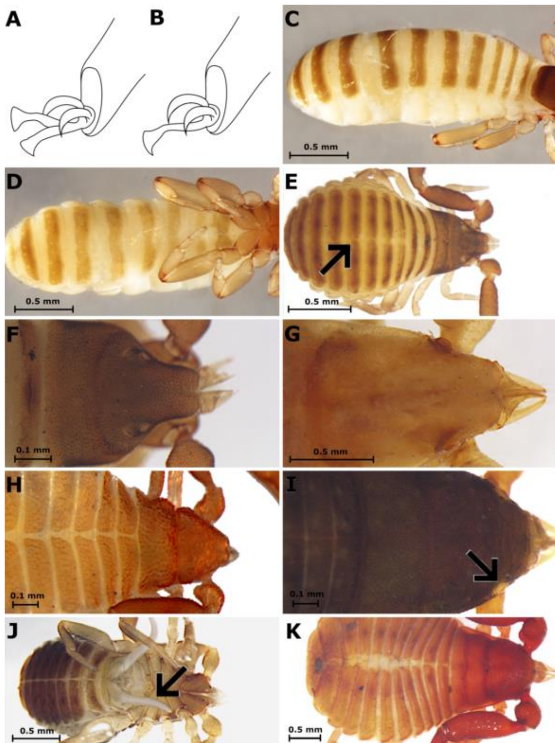
Figure 8. (A). Bifurcate arolia. (B). Simple arolia. (C). Minniza babylonica with all tergites undivided. (D). Minniza babylonica with all sternites undivided. (E). Geogarypus sp. with five tergites divided. (F). Geogarypus sp. with carapace triangular and medially concave. (G). Garypus beauvoisi with carapace triangular but not medially concave. (H). Cheiridiidae gen. sp. with one medial deep transverse furrow in the coarsely granulate and triangular carapace. (I). Hysterochelifer tuberculatus with eyes positioned near the anterior margin of the carapace. (J). Hysterochelifer tuberculatus with articulation of femur and patella of leg I and II well developed and male genitalia with ram's horn shaped organs. (K). Chernetidae gen. sp. robust with two grooves in the carapace and without eyes or eye spots.
