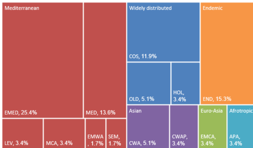
Figure 9. The zoogeographic composition of the pseudoscorpion fauna in Israel. See Table 1 for the chorotype classification and codes.
