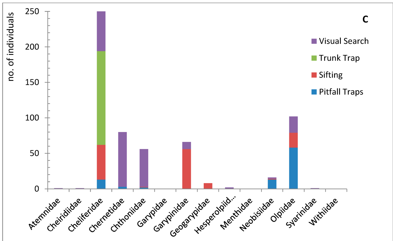
Figure 5. Seasonality, habitat, and collection methodology of pseudoscorpions deposited at the HUI collection. (A) Seasonal distribution of the pseudoscorpion families in Israel (winter: December–February; spring: March–May; summer: June–August; autumn: September–November) (based on the data of 1614 specimens in the collection, Supplementary Materials Table S4). (B) Habitats occupied by pseudoscorpion families in Israel (according to data of specimens in the collection). Data of the same specimen can contribute to more than one category, e.g., desert and under a stone; or cave and related to animals (Supplementary Materials Table S5). (C) Collection method (according to the data of 583 specimens in the collection, Supplementary Materials Table S6).
