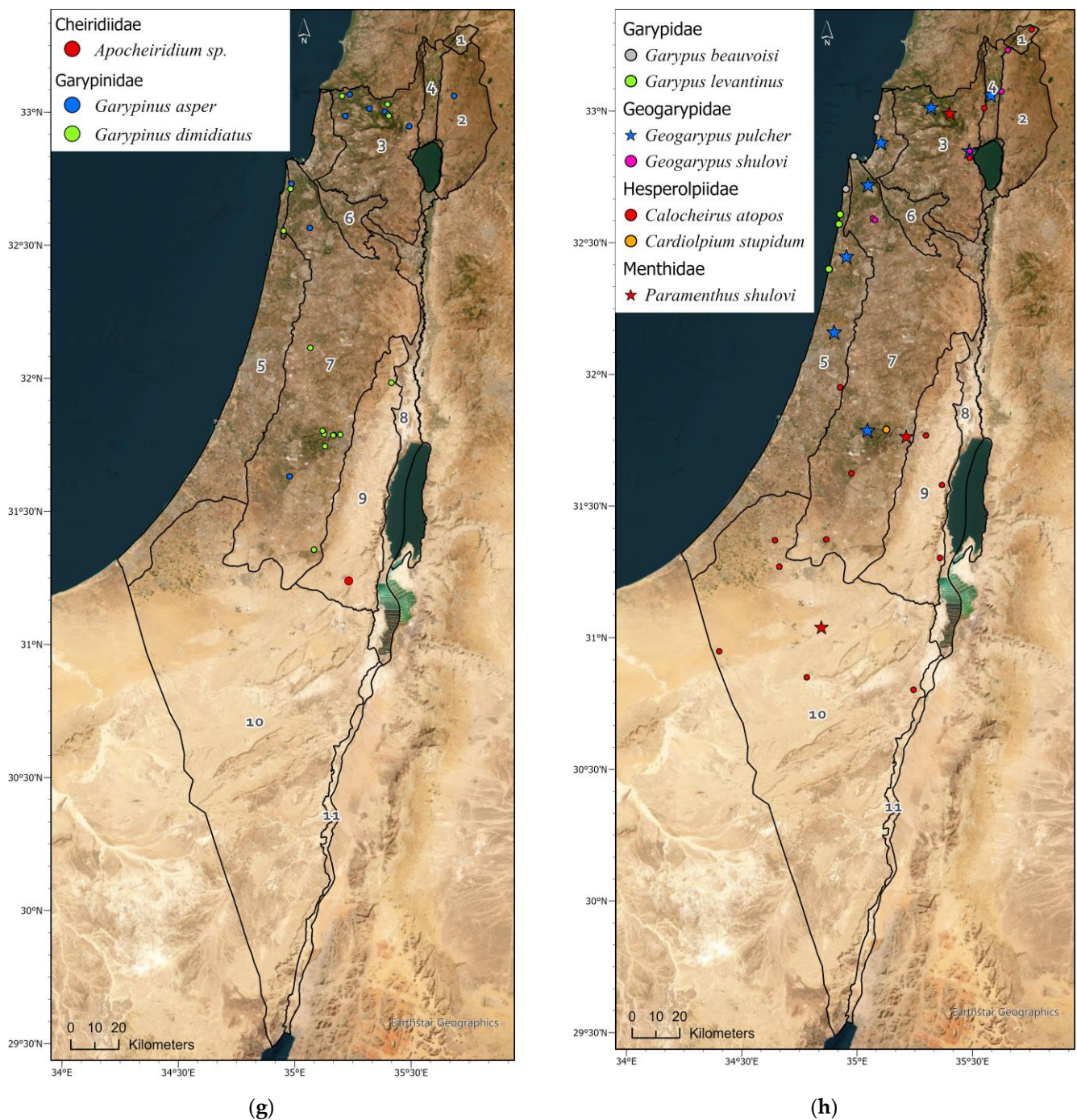
Figure 4. Geographic distribution maps of the pseudoscorpion species in Israel. Localities of 1397 identified specimens deposited in the collection (circle) (Supplementary Materials Table S3), and localities specified in: Beier [15], Halperin and Mahnert [17], Mahnert [16] and Štáhlavský et al. [28] (square). Endemic species are indicated by a star symbol. (a) Cheliferidae; (b) Cheliferidae; (c) Olpiidae; (d) Cheliferoidea (Atemnidae, Chernetidae and Withiidae); (e) Neobisioidea (Neobisidae and Syarinidae); (f) Chthoniidae; (g) Cheiridiidae and Garypinidae; (h) Garypoidea (Garypidae, Geogarypidae, Hesperolpiidae and Menthidae).
