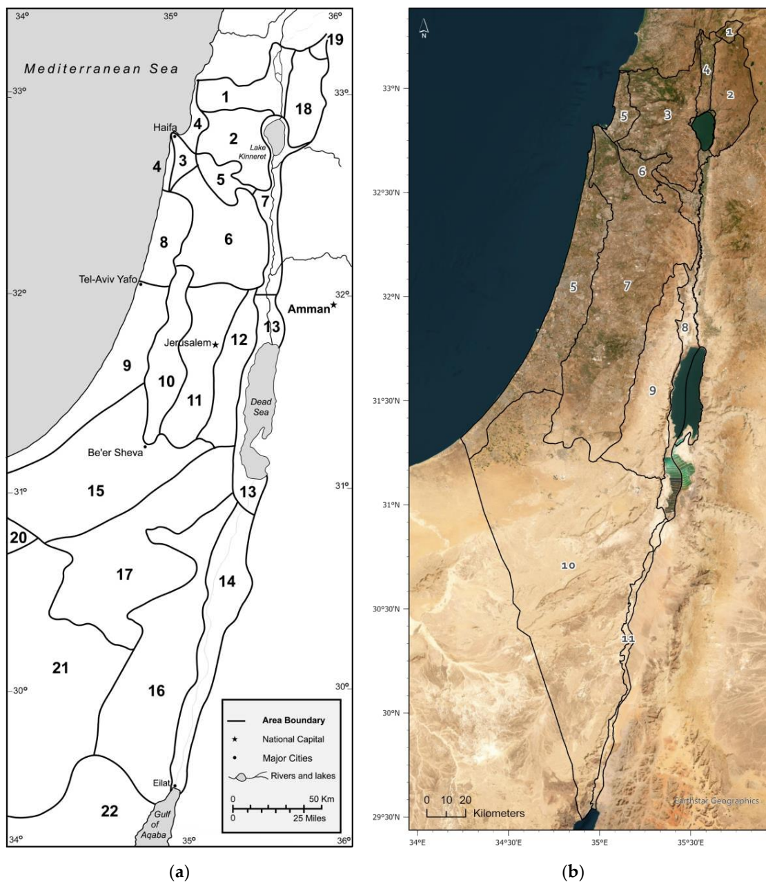
Figure 1. Maps of Israel and adjacent countries. (a) Scheme of biogeographical units in Israel and adjacent countries (adopted from Klein 1988): 1. Upper Galilee; 2. Lower Galilee; 3. Carmel Ridge;
