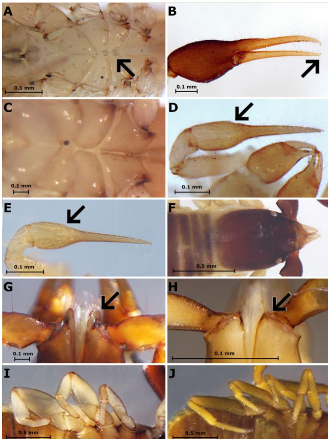
Figure 7. (A). Ephippiochthonius tetrachelatus with coxal spines present. (B). Geogarypus pulcher with venom apparatus on both pedipalpal chelal fingers. (C). Neobisium validum with no coxal spines. (D). Ephippiochthonius sp. with dorsal step-like outline of the pedipalpal hand. (E). Cthonius sp. with evenly rounded weakly curved dorsal outline of the pedipalpal hand. (F). Neobisium validum with five setae on rounded pedipalp coxa apex. (G). Hadoblothrus sp. pedipalp coxal apex not rounded and bears two long subequal setae. (H). Garypinus sp. with the width of the chelicerae bases smaller than the width of the posterior margin of the carapace. (I). Garypinus sp. with two tarsal segments in all legs. (J). Hysterochelifer tuberculatus with one tarsal segment in all legs.
